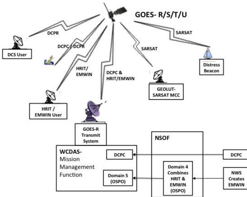
Figure 7: GOES-R Auxiliary Communications Data Distribution System (CCR 1803, CCR 2680A)
