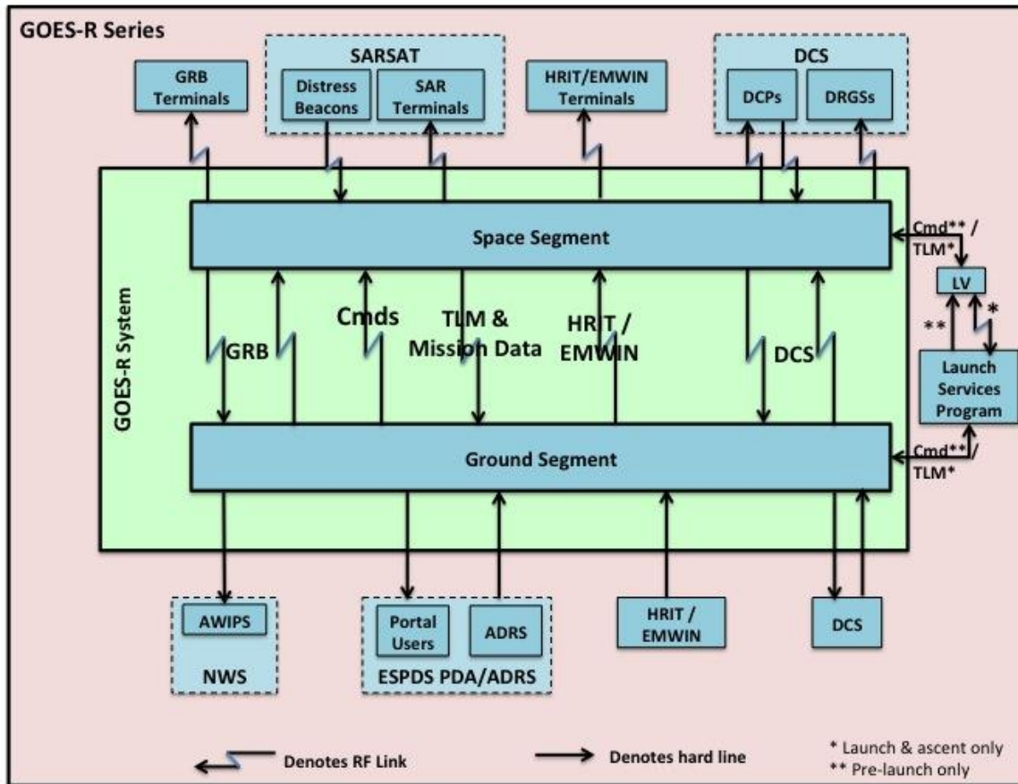
Figure 3 : GOES-R Mission Interfaces (CCR 1558, CCR 1803, CCR 2680A)
