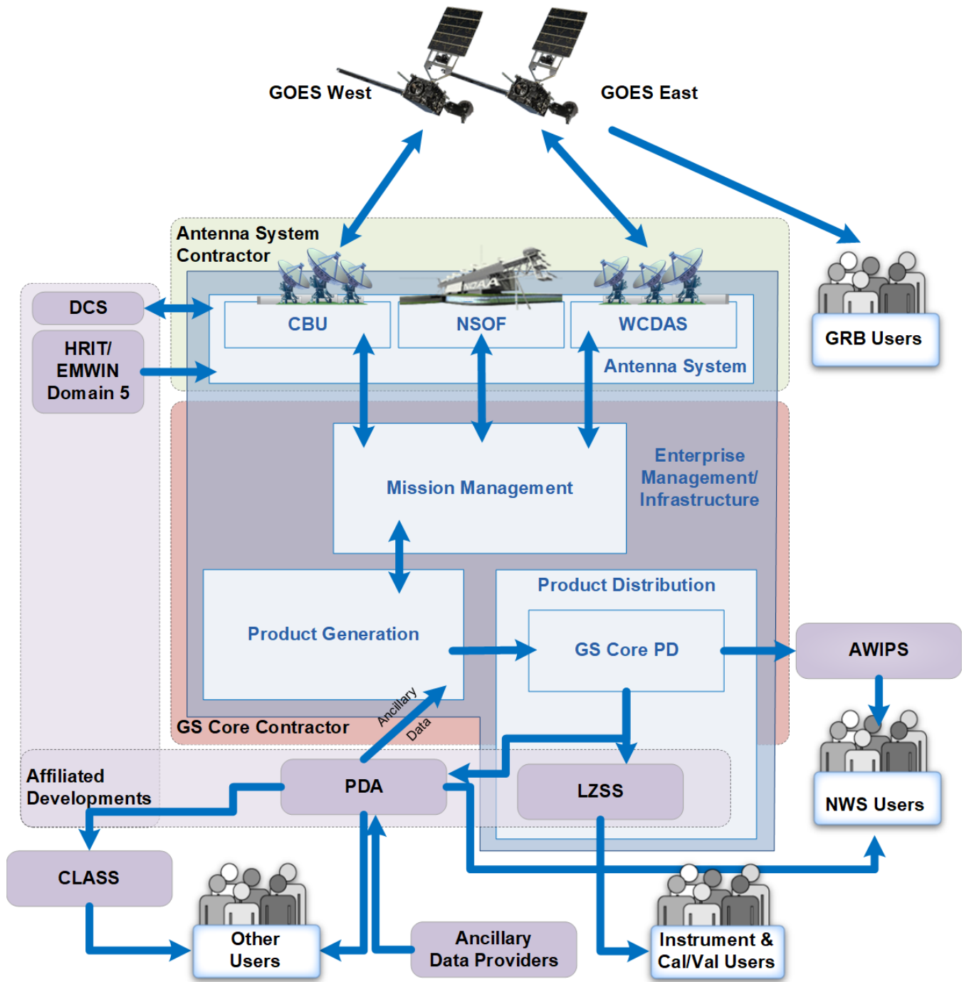
Figure 6: GOES-R Data Distribution System (CCR 1558, CCR 1803, CCR 2680A, CCR 2838, CCR 3584)
