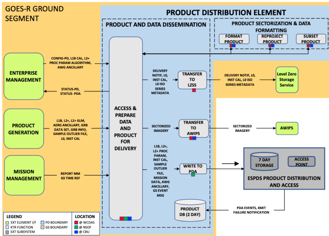
Figure 5: Product Distribution (PD) and Primary External Interfaces (CCR 1558, CCR 1803, CCR 2680A, CCR 2838, CCR 3584) CCOR PD not shown here
