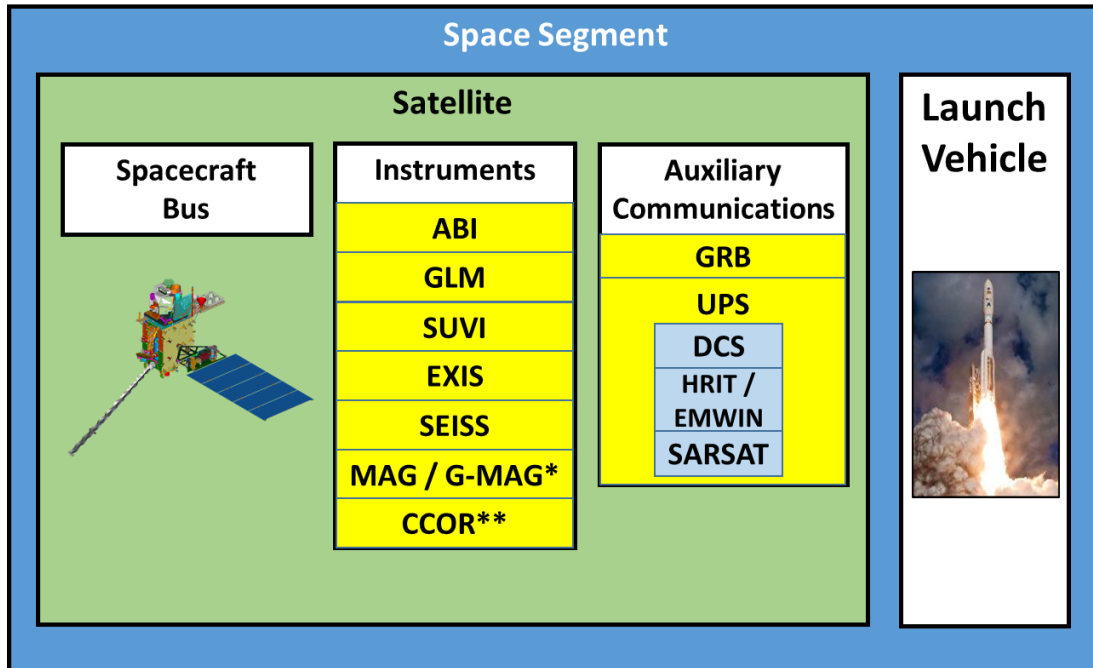
Figure 4: GOES-R Space Segment Composition (CCR 1558, CCR 3584)
